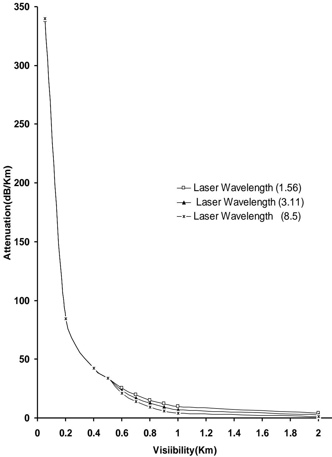
Figure (γ) Atmospheric Attenuation as a function of the Visibility for different Laser wavelength.
